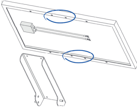
20 W / 40 W solar panel
