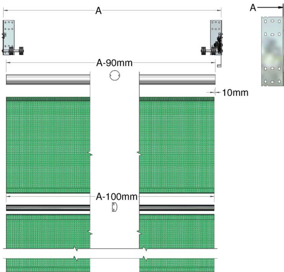
Figure 4a, Standard Cutting Lengths of Tubes and Fabric
