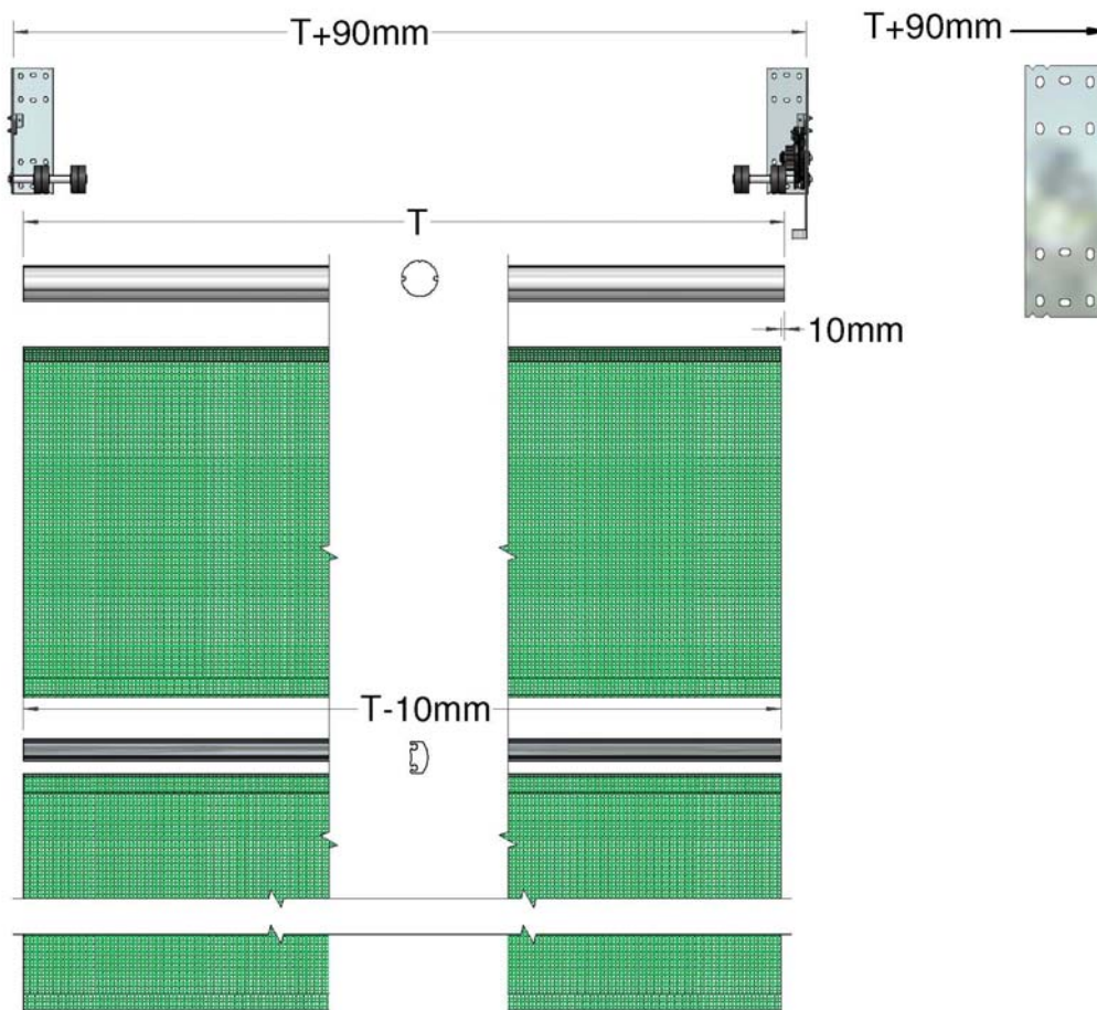
Figure 4b, Top Bracket Spacing When Not Cutting Tube, Windbars and Fabric
