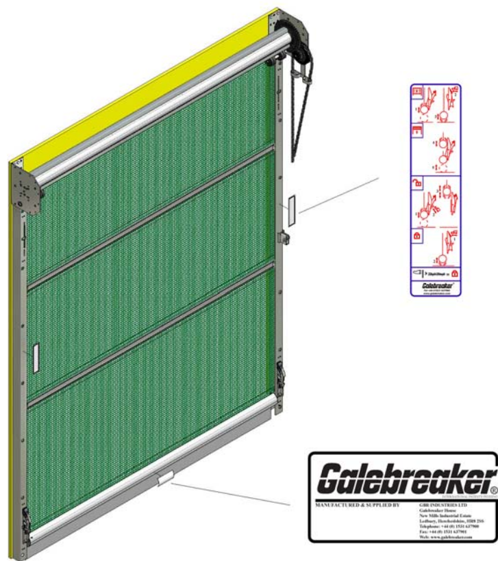
Figure 18, Attaching Labels
