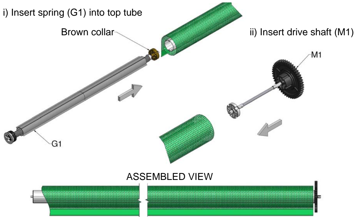
Figure 6c, Top Tube Assembly (Right Hand Drive)
