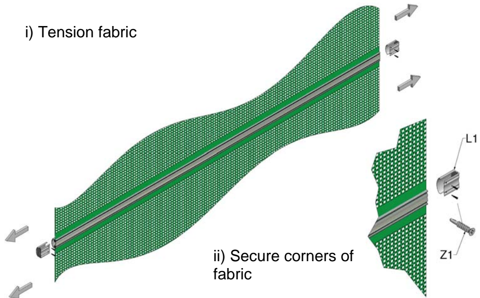
Figure 5c, Securing Fabric
