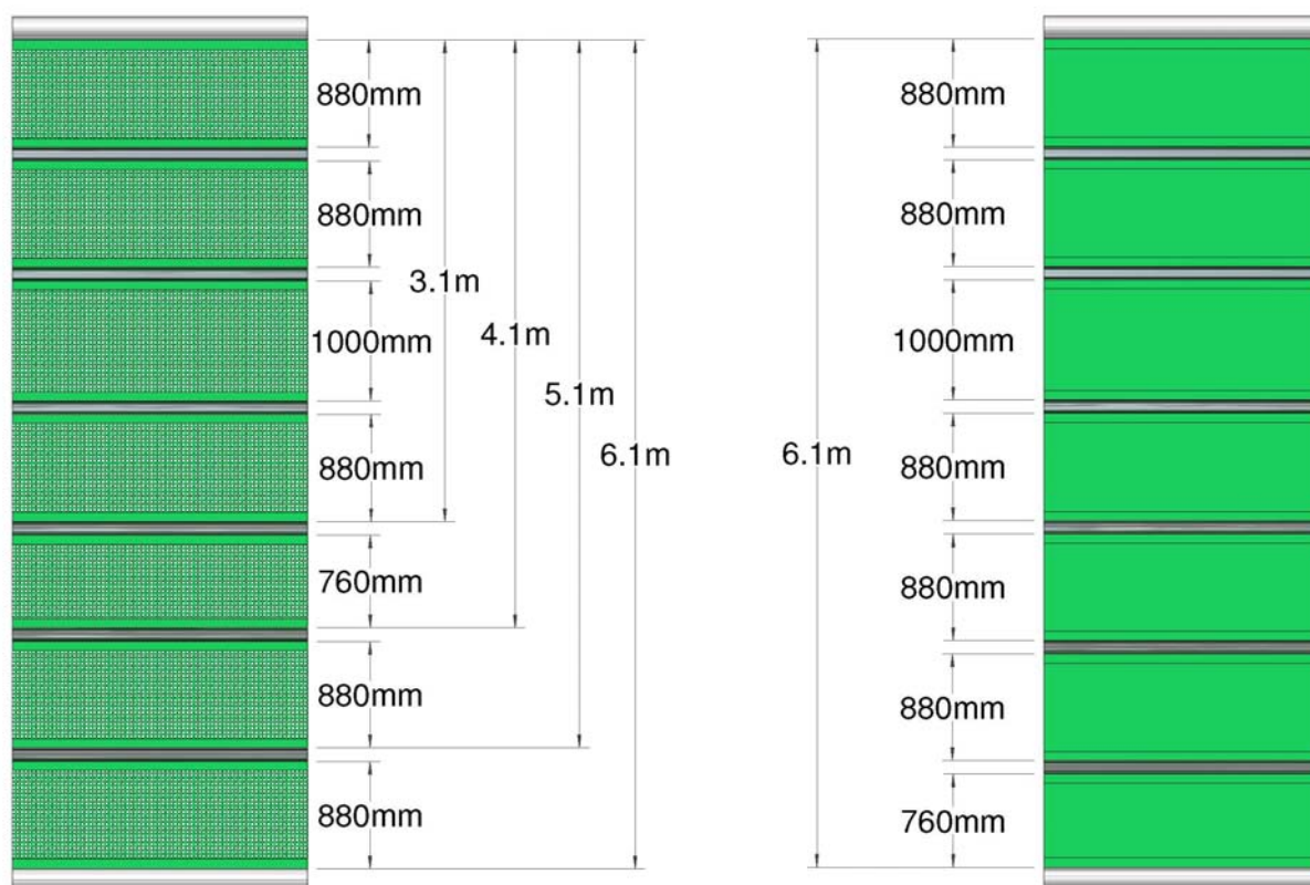
Figure 5b, Fabric Panel Layout
