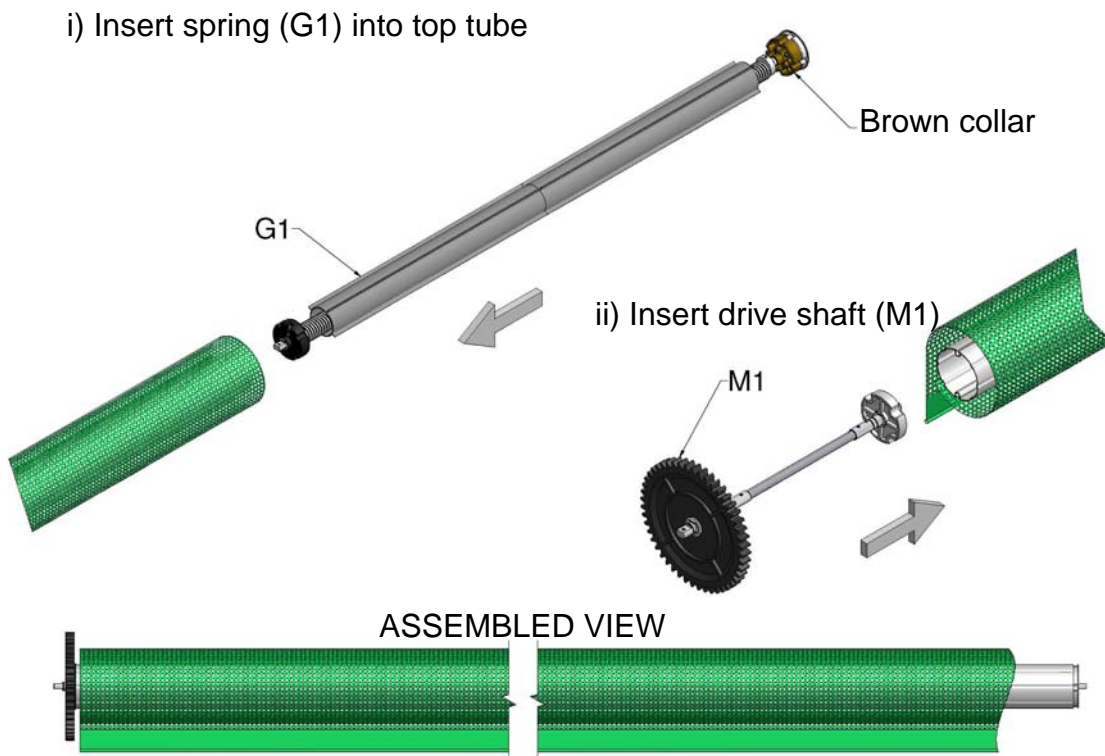
Figure 6d, Top Tube Assembly (Left Hand Drive)
